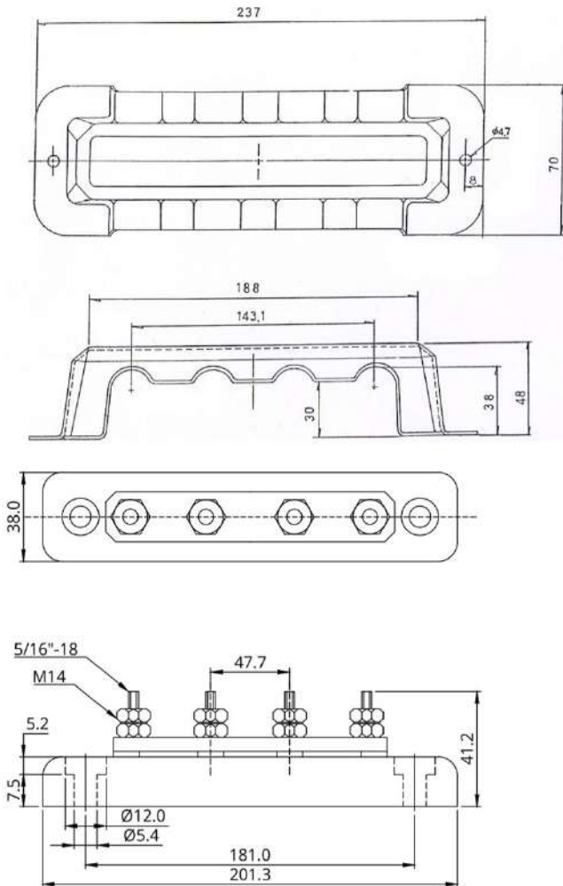
Busbar 250 A with 4 stud terminals and cover
