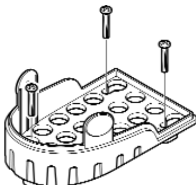
Fig 5 Connect Strainer IC to bulkhead
